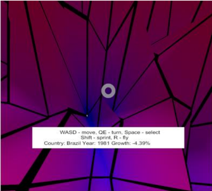
Figure 29 Cursor border
