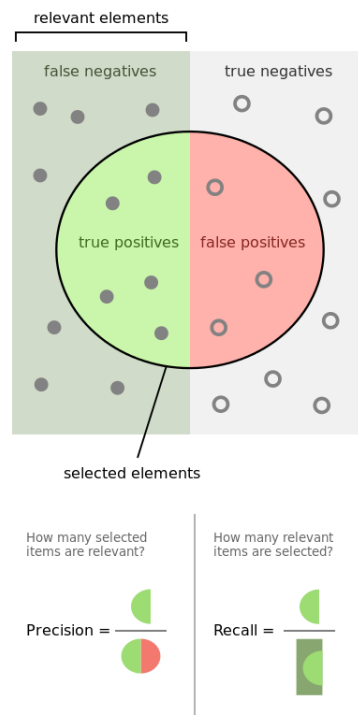
FIGURE C.1 – Source : https://commons.wikimedia.org/wiki/File:Precisionrecall.svg
