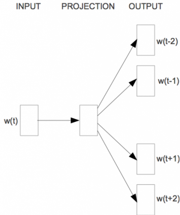
FIGURE 2.4 – Architecture skip-gram
