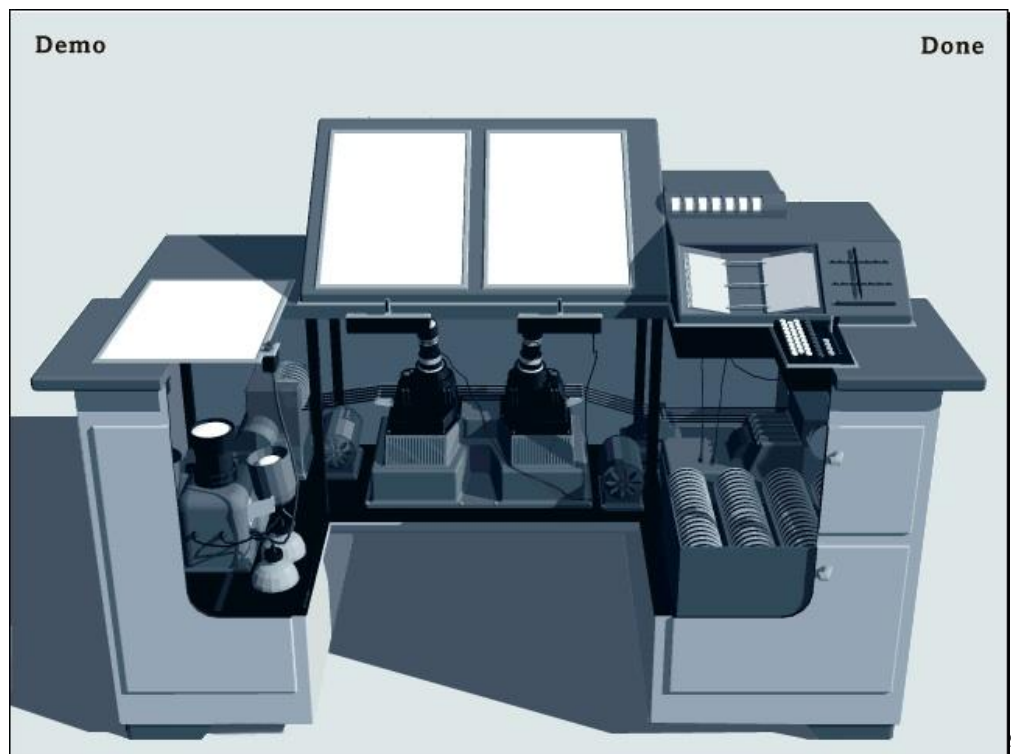
Figure 1: Le Memex
